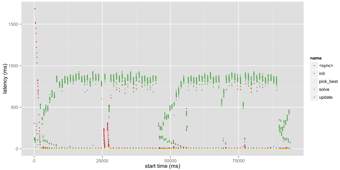
Figure 3: Task execution times for 30 ants
