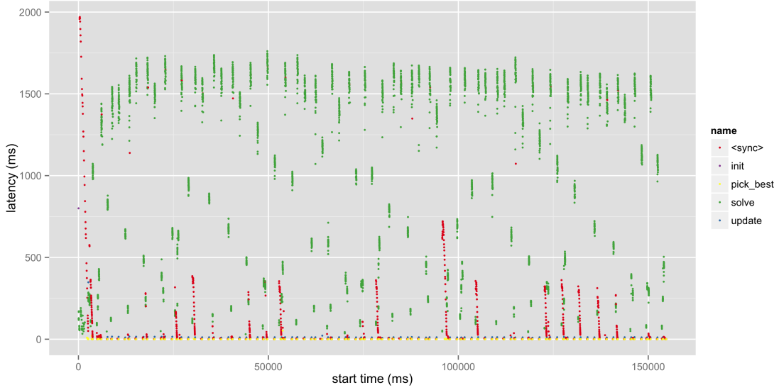
Figure 2: Task execution times for 40 ants
