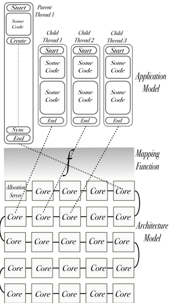
Figure 1: High-level simulation of the microthreaded architecture
